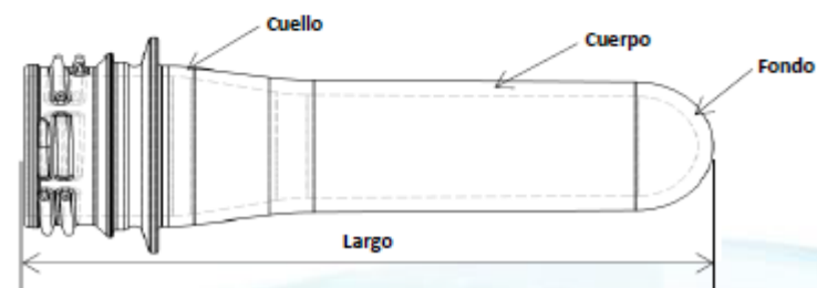
Rosca Baja PCO 1881 – 28mm
