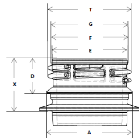
Rosca Baja PCO 1881 – 28mm
